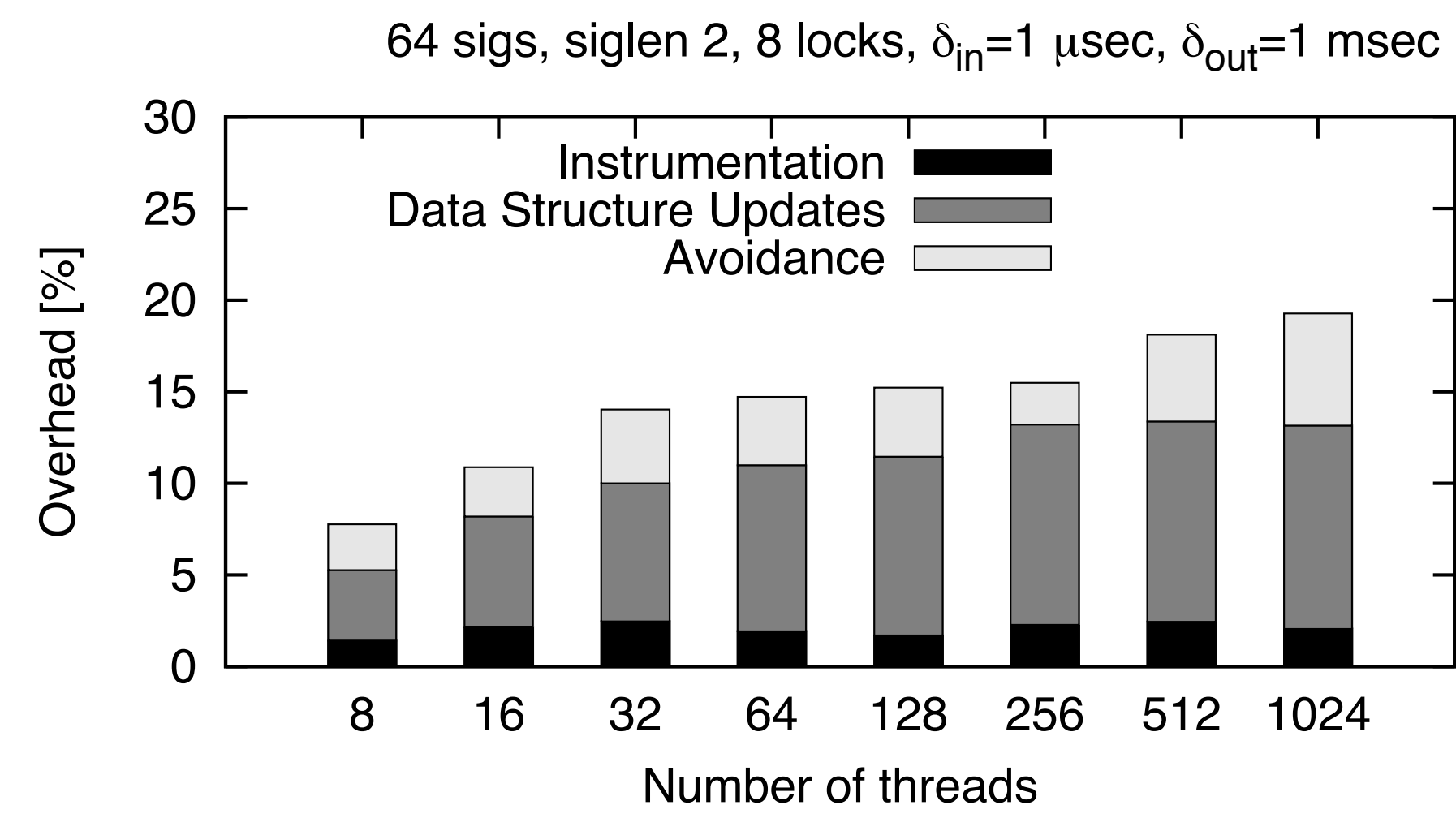
Figure 8: Breakdown of overhead for Java Dimmunix.
