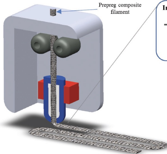
(a) Fused Filament Fabrication
