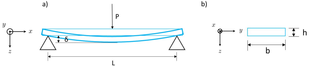
Figure 1: a) Three point bending test showing the applied load P , the span L and the deflection of a beam \delta , and b) rectangular cross section of the beam, with height h and width b .
