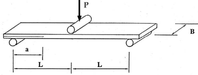
Figure 8: Configuration of the delamination test in mode II, with applied load P , crack length a , beam length 2L , and width B .
