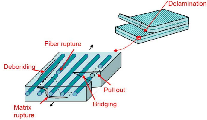
Figure 4: Different modes of composite damage.
