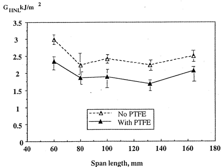
Figure 5. Results for G_{IINL} from mode II tests on 5.2-mm-thick specimens, with and without PTFE separator. Error bars show maximum and minimum values measured.
