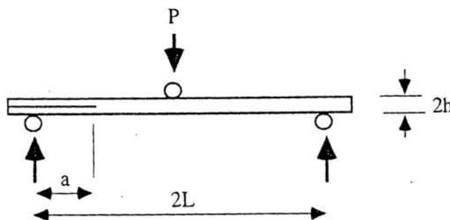
Figure 1. Specimen configuration.
