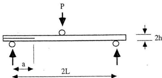
Figure 1. Specimen configuration.
