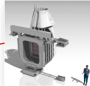
BEAM SOURCE
