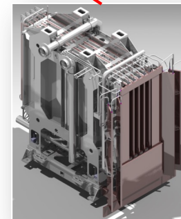
NEUTRALIZER
