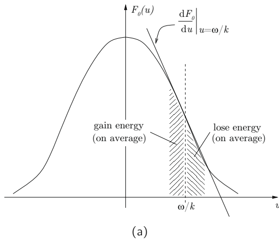
Figure 5: (a) Particles with u \lesssim \omega/k will gain energy from the wave and particles with u \gtrsim \omega/k will lose energy to the wave. As there are more particles which gain energy, the overall effect is that the wave is damped.
