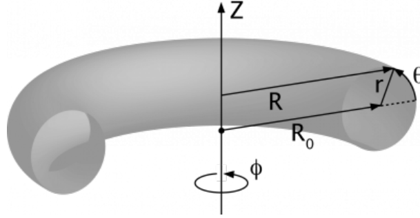
Figure 1: Toroidal coordinates.
