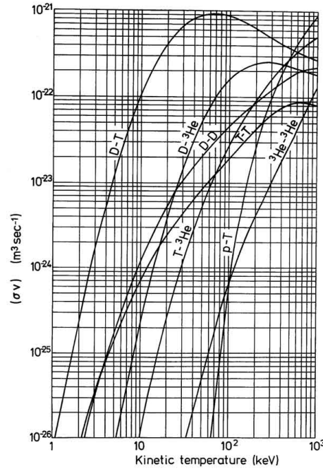
Figure 3: Fusion \langle \sigma v \rangle_{DT} as a function of the plasma temperature.
