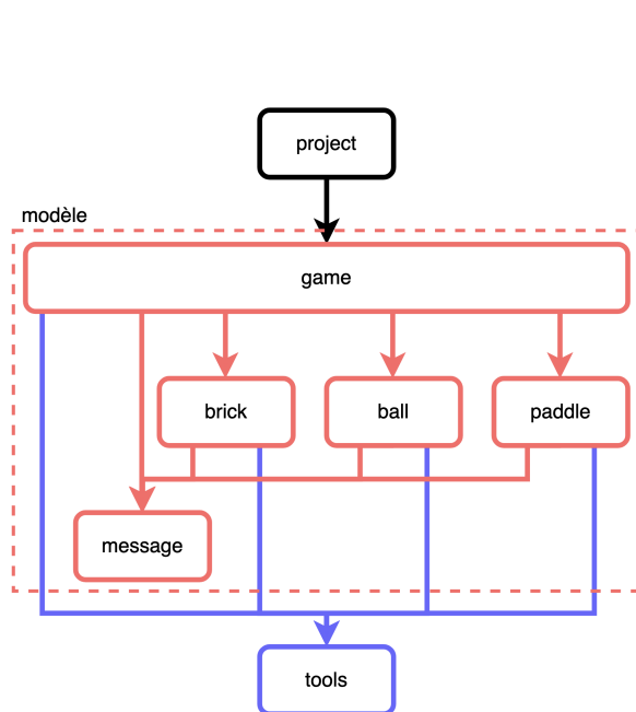
FIGURE 11 – Architecture sans interface graphique (rendu 1)
