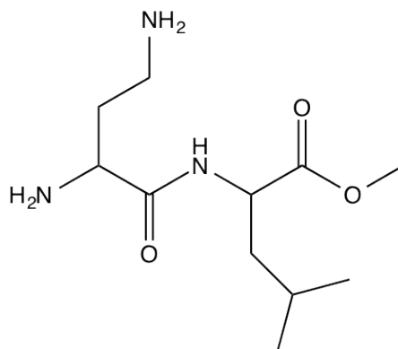
methyl (2,4-diaminobutanoyl)leucinate
