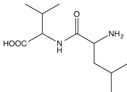
leucylvaline
