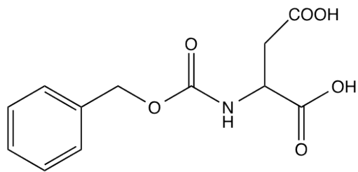
((benzyloxy)carbonyl)aspartic acid
