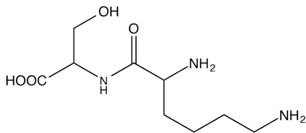
lysylserine
