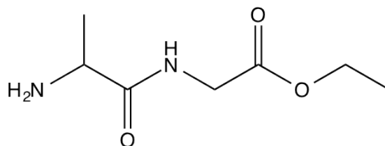
ethyl alanylglycinate
